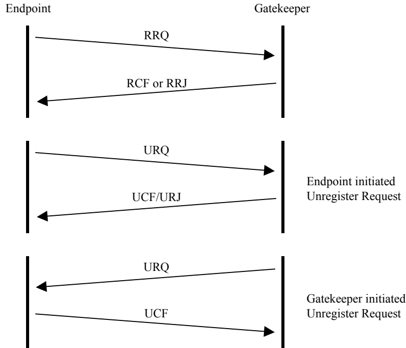
Figure 8 - Endpoint registration
