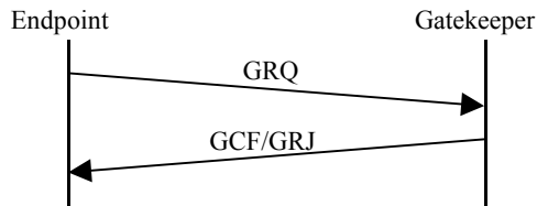
Figure 7 - Gatekeeper autodiscovery
